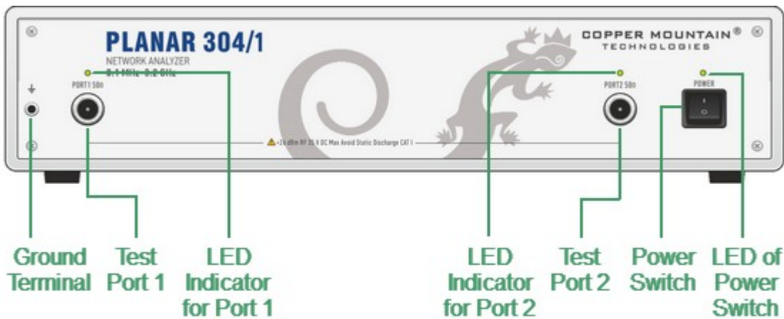
Full-Size 304/1 front panel
