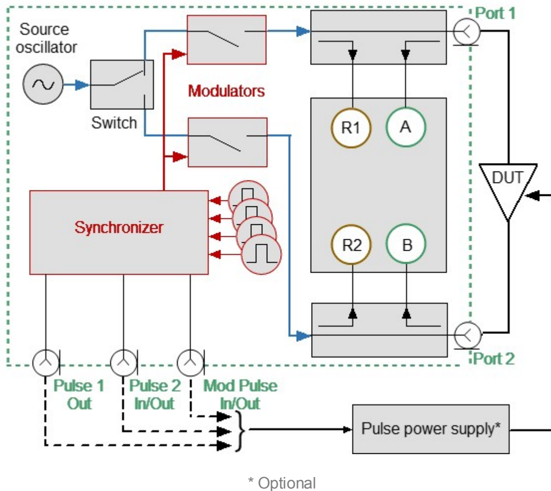
Pulse-in-pulse with internal trigger
