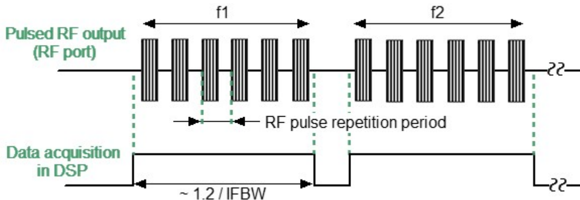
Asynchronous pulse
