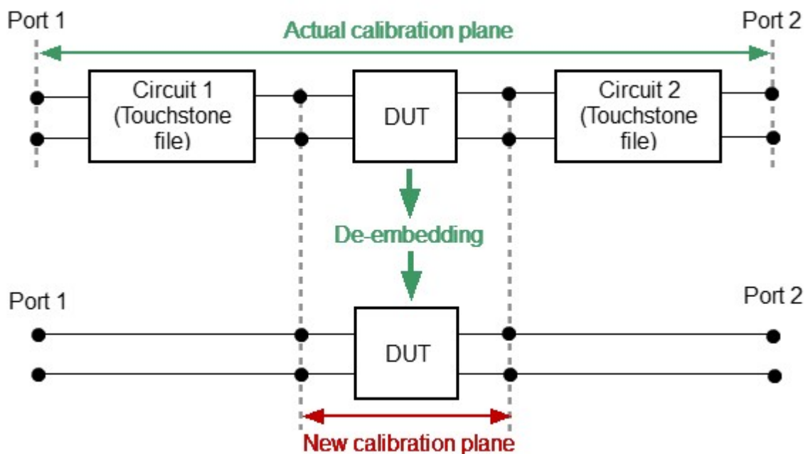
De-embedding process
