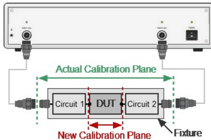
De-embedding
