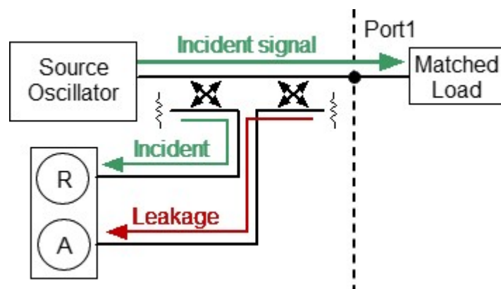
Directivity error
