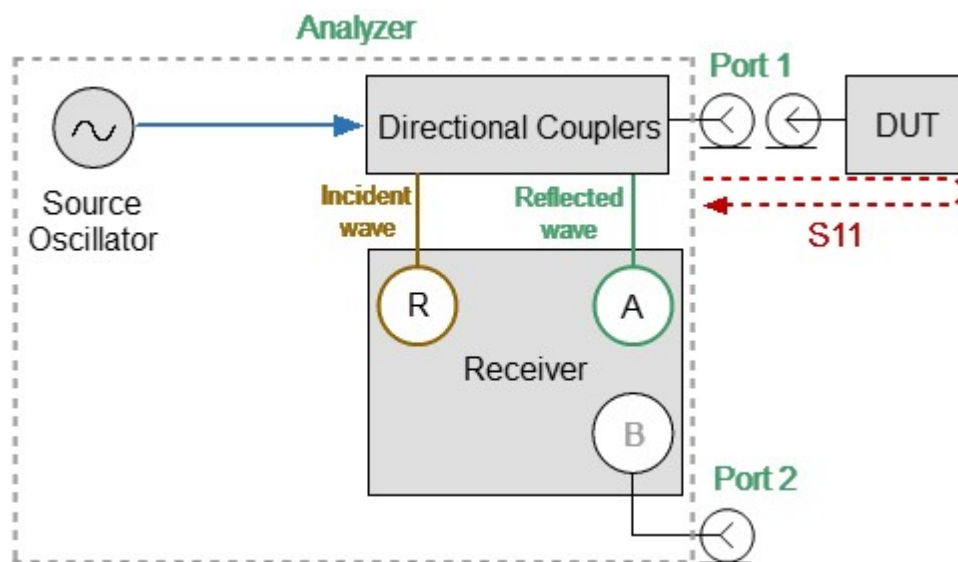
Reflection Measurement
