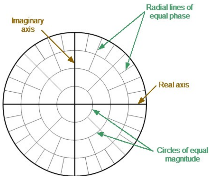
Polar format
