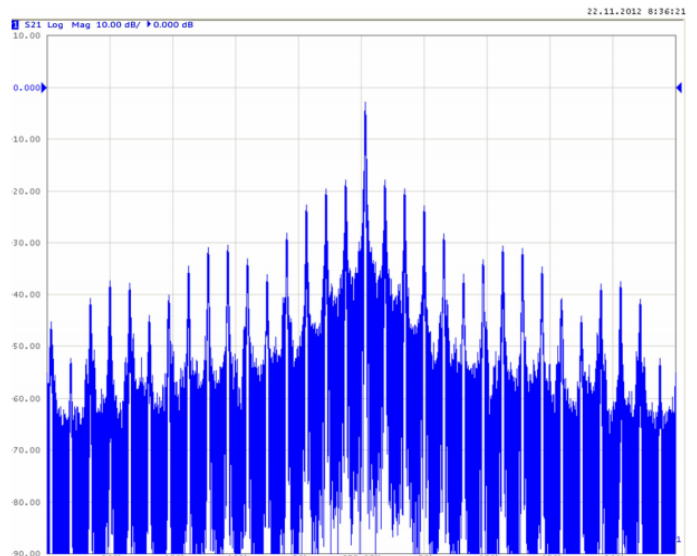
Figure 8: Analog TV signal, Measurement Bandwidth – 0.5 MHz.
