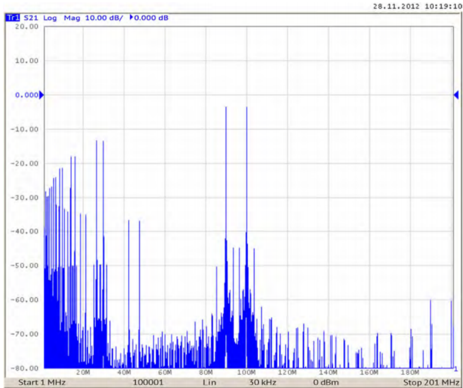
Figure 1: Filtered signal 100 MHz and its harmonics. Measurement bandwidth 200 MHz *
