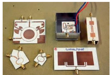
Implemented microwave components of a radar module
