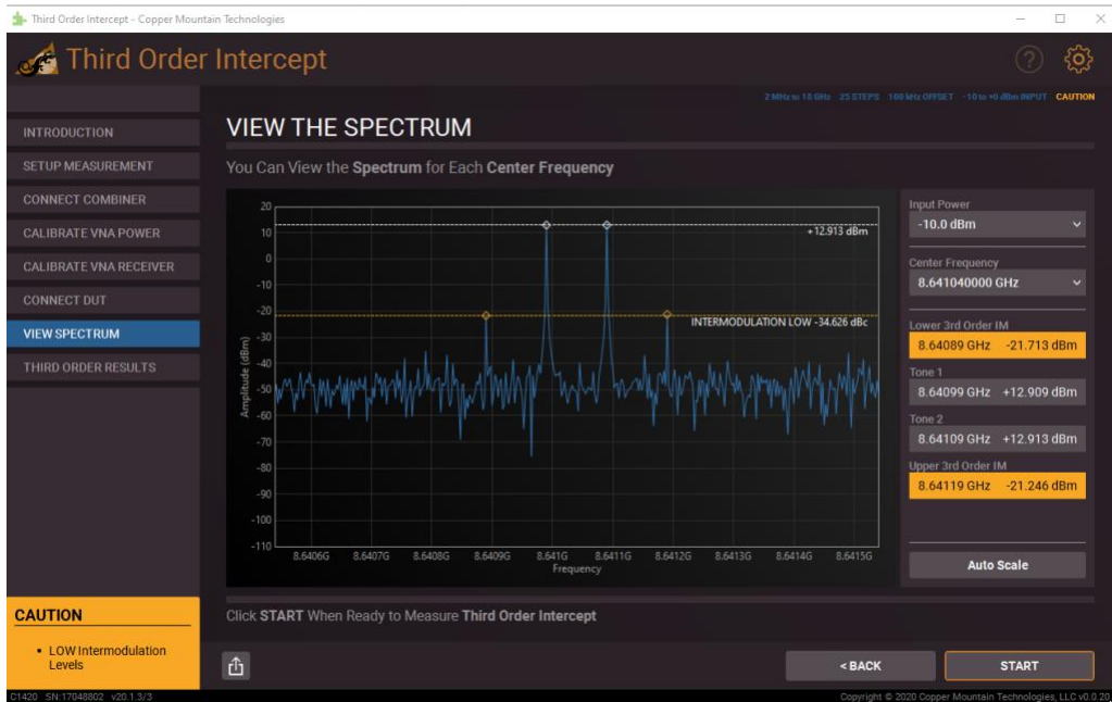
Figure 6: Spectrum Measurement
